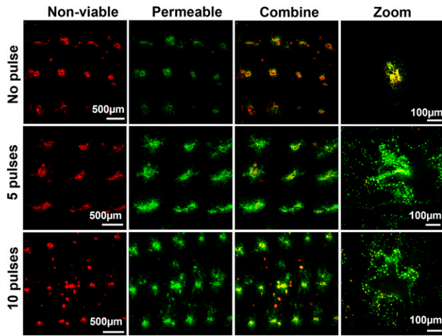
Fig. 5. Cell membrane permeabilization and cell viability in mouse skin in vivo after electroporation by ePatch. Representative images show nonviable cells (red color) and cells with permeabilized membrane (green color) in the skin after electroporation with 0, 5, or 10 pulses by ePatch. Nonviable cells were identified in the mouse skin after insertion of MEA without electroporation (no pulse), suggesting that a small number of cells were damaged by microneedle electrode insertion alone. The red and green signals are colocalized in the insertion holes because nonviable cells are also permeable to the SYTOX Green. After 5 and 10 pulses, the red signal did not increase in the skin, while the green signal became more dispersed in the skin, suggesting transient cell permeability induced by the piezoelectric pulses with little effect on cell viability.
