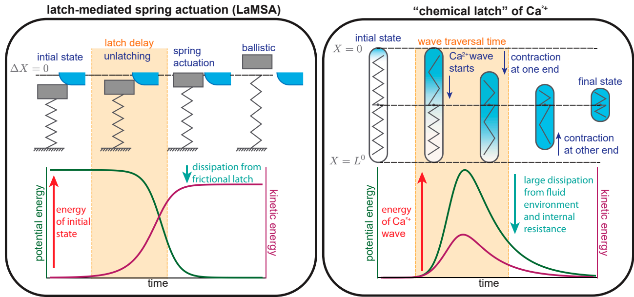
Fig. 6. Schematic illustration of a chemical latch. The Left panel, adapted from ref. 68, illustrates a mechanical latch-and-spring system. A latch, shown in blue, slides frictionally off of a compressed spring, shown in gray, which allows for a fast release of the stored potential energy. The finite time during which the latch slides is highlighted in orange. The potential and kinetic energies of the system are schematically plotted at the bottom. At smaller scales, such as the scale of a single-cell organism like Spirostomum , a different paradigm accounts for the chemical nature of mechanical activation (via a traveling \text{Ca}^{2+} wave). This is illustrated in the Right panel, where analogous features of the dynamics in the macroscopic case are shown in the corresponding colors. The traveling wave is shown as a blue gradient, which controls the local rest length (indicated as the number of ridges) of internal springs, shown in gray.
